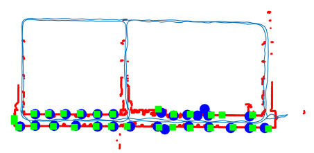
Fig. 5: Estimated trajectory in second office experiment from our algorithm (blue line) along with our estimated door landmark positions (blue circles), overlaid onto partial ground truth map (red) along with ground truth door locations (green squares)
