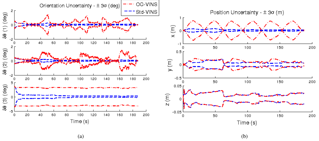
Figure 4: Comparison of the estimated 3\sigma error bounds for attitude and position between Std-VINS and OC-VINS.
