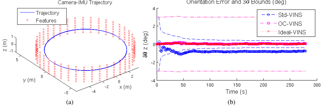
Figure 1: (a) Camera-IMU trajectory and 3D features. (b) Error and 3\sigma bounds for the rotation about the gravity vector, plotted for a single run.
