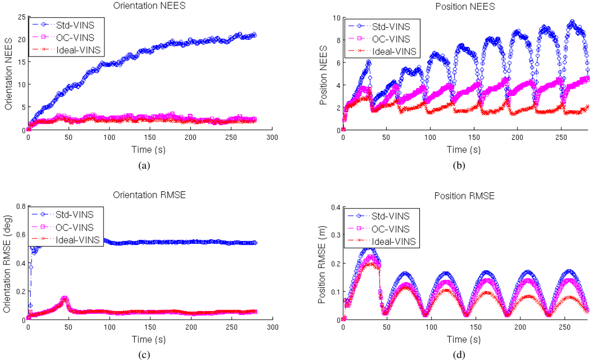
Figure 2: The RMSE and NEES errors for position and orientation plotted for all three filters, averaged per time step over 100 Monte Carlo trials.
