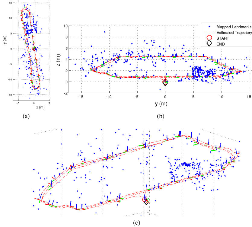
Figure 3: The estimated 3D trajectory over the three traversals of the two floors of the building, along with the estimated positions of the mapped landmarks. (a) projection on the x and y axis, (b) projection on the y and z axis, (c) 3D view of the overall trajectory and estimated features
